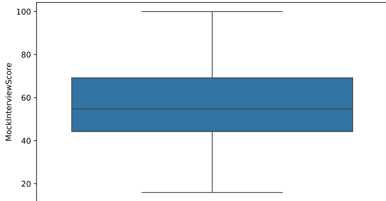
MockInterviewScore
